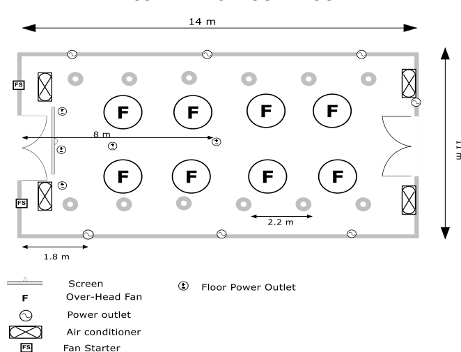
INDABA CONFERENCE ROOM FLOOR PLAN
