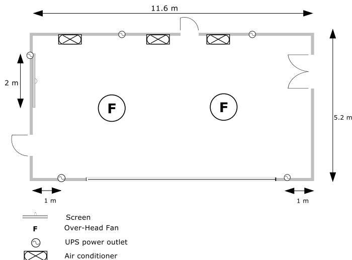
BOARDROOM FLOOR PLAN
