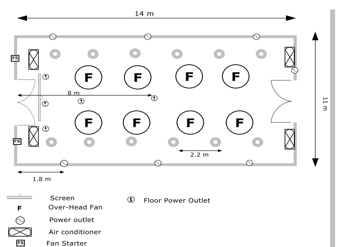
INDABA CONFERENCE ROOM FLOOR PLAN
